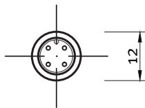
connector view 4 pin M 12 x 1 RSFM 5
