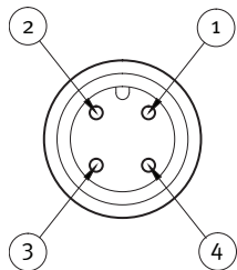
connector view 4 pin M 12 x 1 RSFM 5
